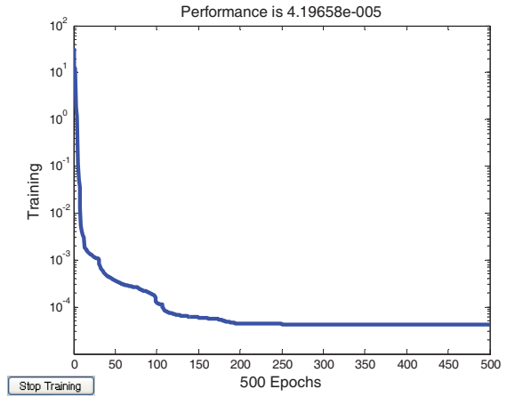
Fig. 10. Training result of neural network for 2-phase faults
