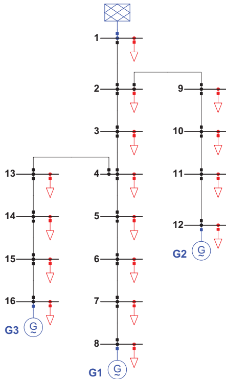
Fig. 7. The studied distribution network
