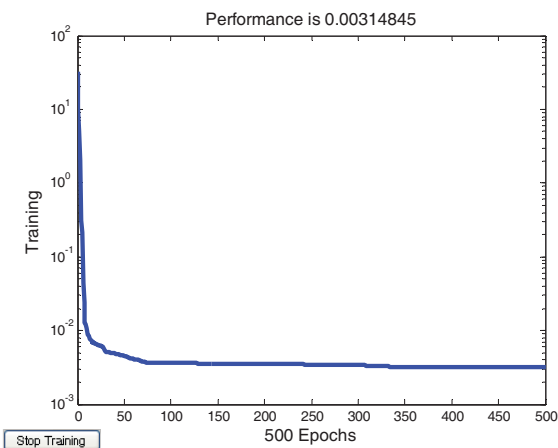
Fig. 9. Training result of neural network for 1-phase faults
