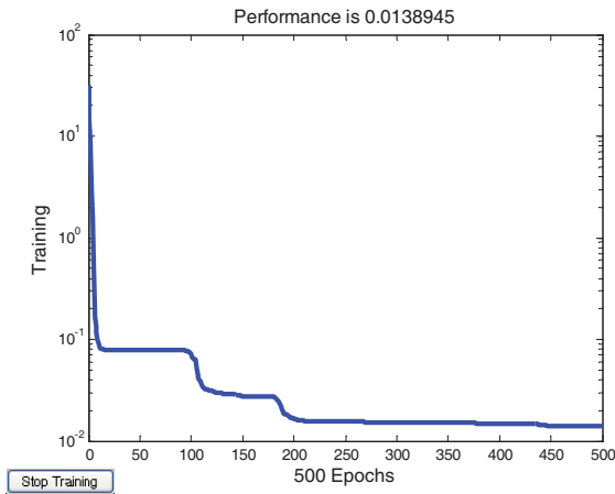
Fig. 8. Training result of neural network for 3-phase faults
