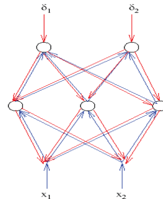
Fig. 3. Standard back propagation training method
