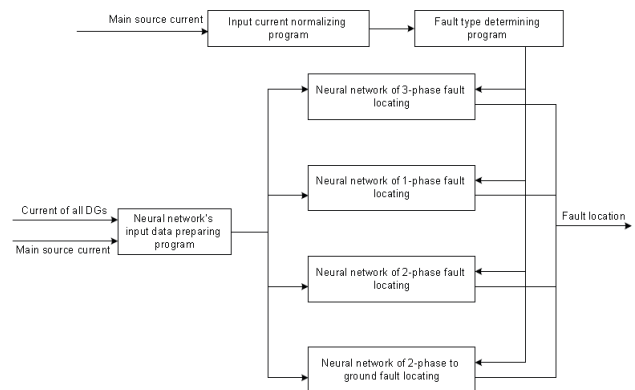
Fig. 4. The outline of the proposed method
