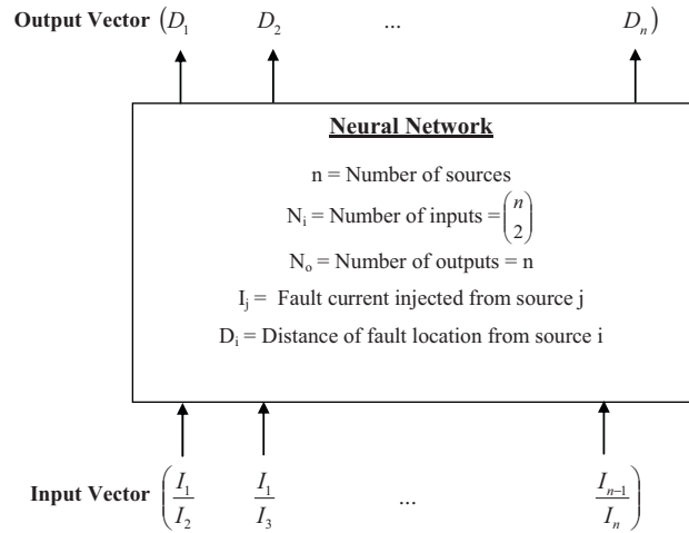
Fig. 6. The structure of neural network
