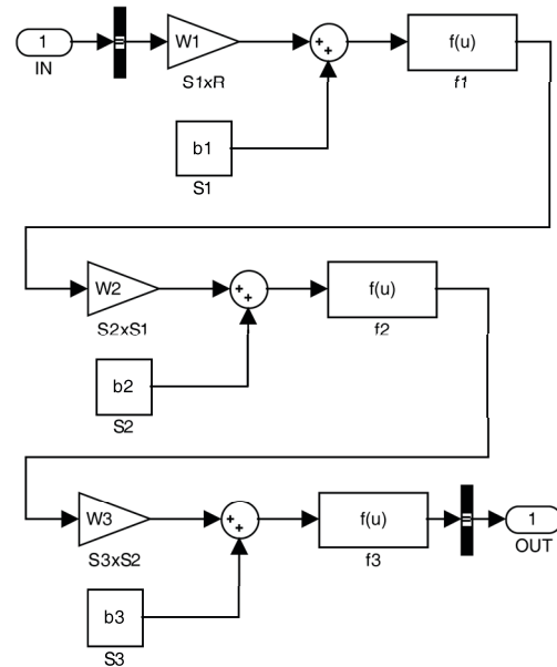
Fig. 2. The block-diagram of a 3-layer Perceptron
